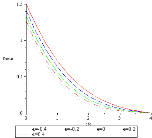
Fig.3. Variation of the non-dimensional temperature as function of \eta for various values of \epsilon
