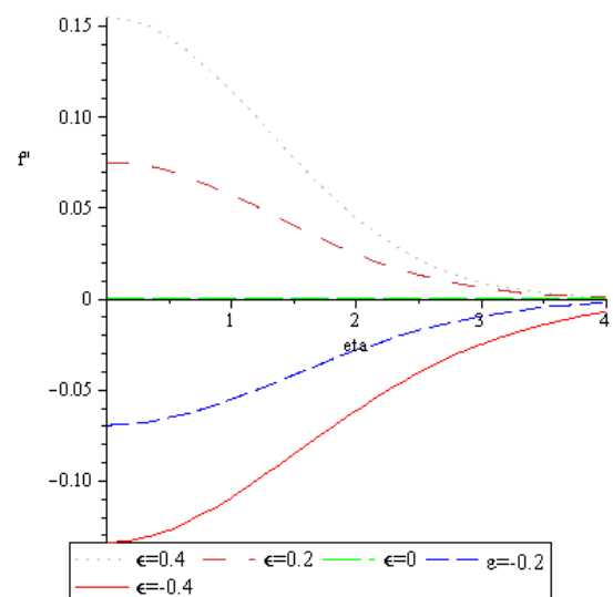
Fig.2. Variation of the velocity gradient as a function of \eta for various values of \epsilon
