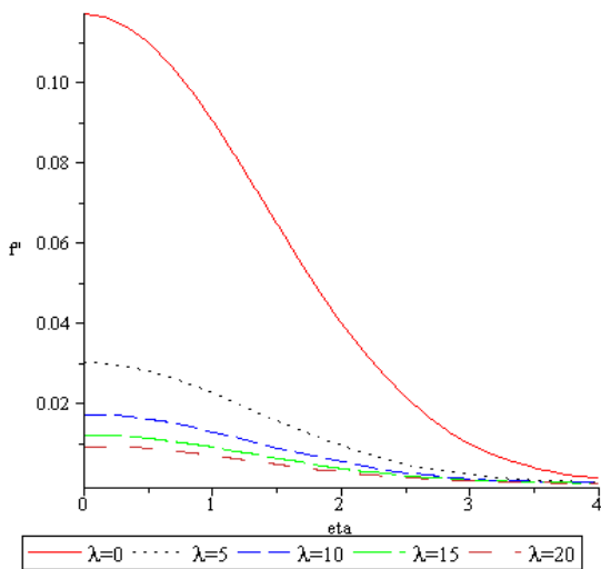
Fig.5. Variation of the velocity gradient as function of \eta for various values of \lambda
