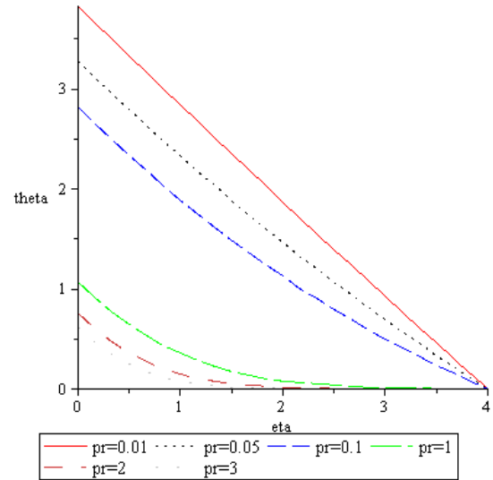
Fig.6. Variation of the non-dimensional temperature as function of \eta for various values of Prandtl
