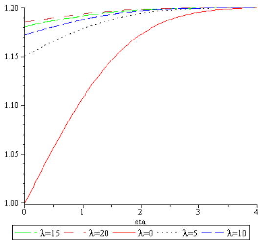
Fig.4. Variation of the velocity profile as function of \eta for various values of \lambda
